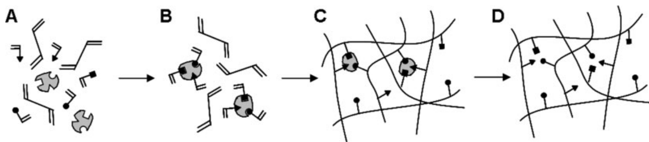
Figure 2. (A) Solution mixture of template, cross-linking monomer, and functional monomers (triangles, squares, circles), (B) Complex formation between functional monomers and template via covalent or noncovalent chemistry, (C) The formation of the polymer network typically via free radical polymerization, and (D) Template removal step which leaves binding sites specific to the original template.
