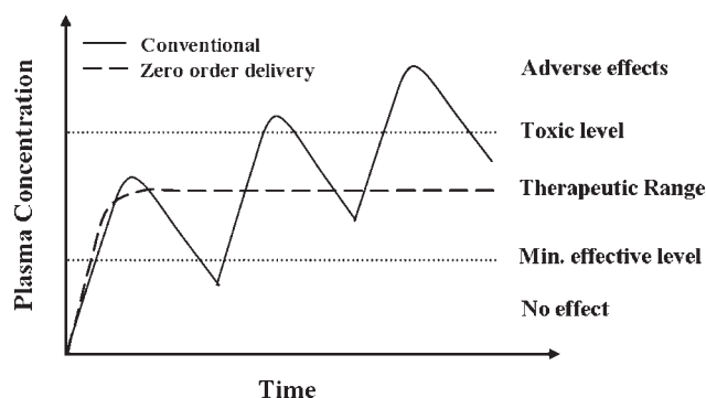
Figure 3. Conventional drug delivery (solid line) involves taking frequent high concentration doses of a therapeutic which often results toxic levels in the body.
